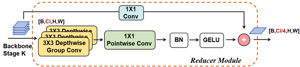
Fig. 2. Reducer module.
