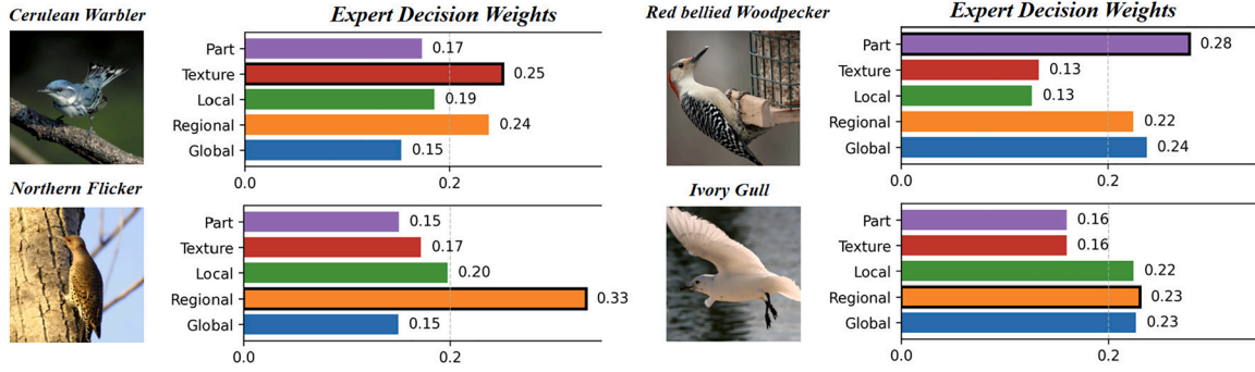
Fig. 9. Dynamic expert allocation for different images.
